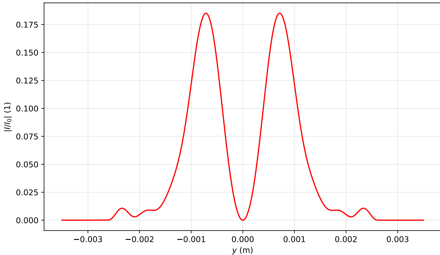
Intensity profile I(x=0, y, z=2.946)/I_0 , \text{Pin}=4.0\text{Pcr} , artificial time
